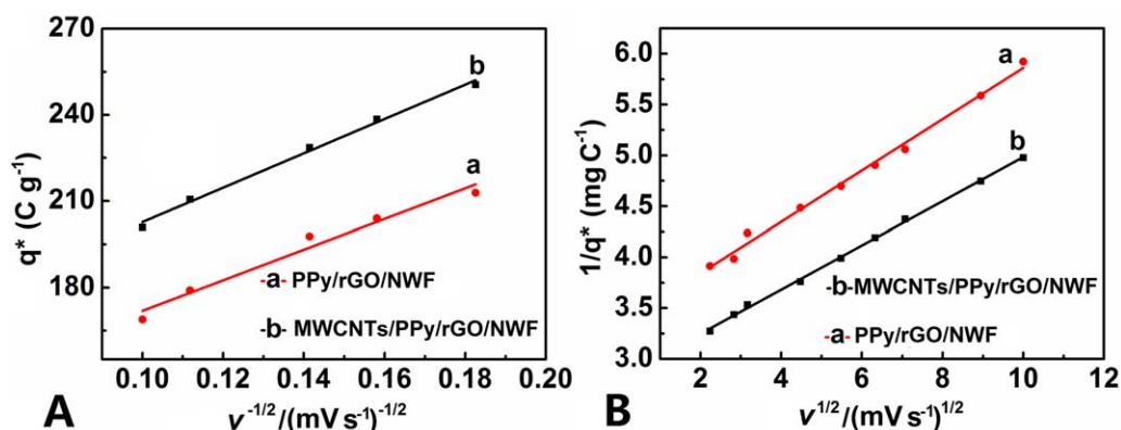
Figure 10. (A) The plots of charge ( q^* ) determined by voltammetric versus inverse square root of scan rate ( \nu^{-1/2} ) and (B) the inverse charge ( 1/q^* ) versus square root of scan rate ( \nu^{1/2} ). [Color figure can be viewed in the online issue, which is available at wileyonlinelibrary.com .]
