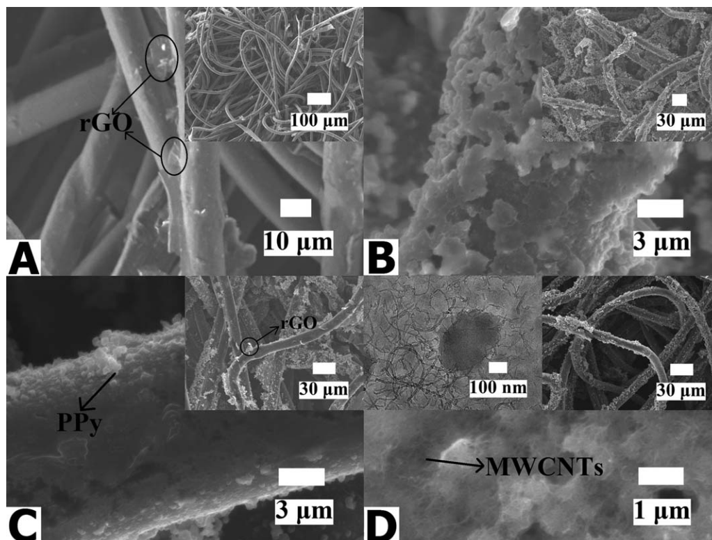
Figure 3. The SEM images of rGO/NWF (A), PPy/NFW (B), PPy/rGO/NWF (C), and MWCNTs/PPy/rGO/NWF (D). The inserted figures are the SEM images in low magnification and TEM image.
